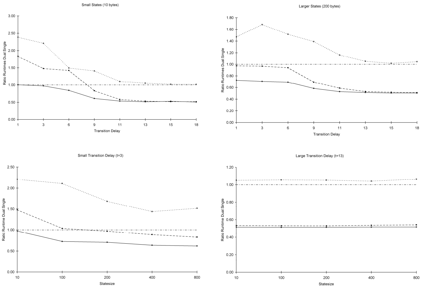
Fig. 6. Measurements on a reference model, to study the effect of structural model properties on the performance of multi-core verification algorithms. Varied are the out-degree of states (the branch factor), the state size, and the transition delay. The dotted, dashed, and solid lines correspond to branch factors of 1 (i.e., a deterministic), 2, and 8 respectively. The horizontal dash-dot line at 1.0 in each graph, indicates the value for which the dual-core runtime equals the single-core runtime (i.e., there is no speedup or slowdown).
