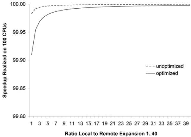
Fig. 2. Effective speedup as a function of IR on a multi-core system, using data from Table II. The relative time to generate a new state is set to 1 for an optimized system and to 50 for an unoptimized system.
