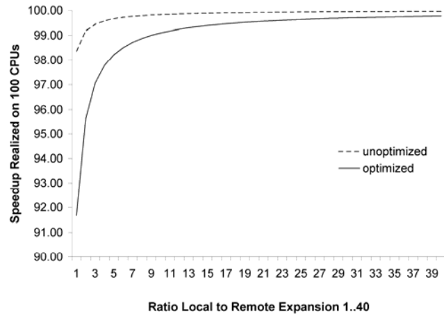
Fig. 1. Effective speedup as a function of IR on a multi-CPU system, using data from Table II. The relative time to generate a new state is set to 1 for an optimized system, and to 50 for an unoptimized system.
