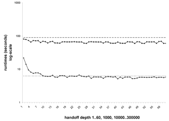
Fig. 5. Dual-Core and Single-Core with (bottom) and without (top) partial order reduction enabled, for varying handoff depths. All runs were compiled with compiler optimization. The performance of the single-core verification runs is indicated by the horizontal lines. Without partial order reduction there are 32.8 Million reachable states; with partial order reduction enabled the number is 4.7 Million states.
