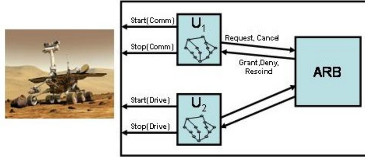
Fig. 6. MER Architecture
