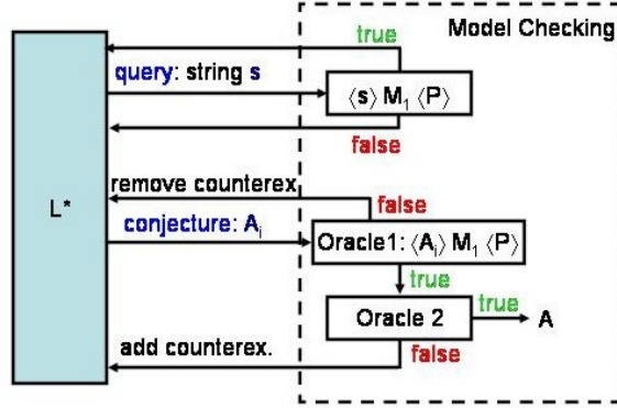
Fig. 2. Tool Architecture
