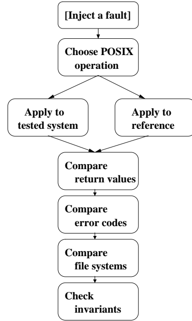
Figure 1. Randomized differential testing inner loop
