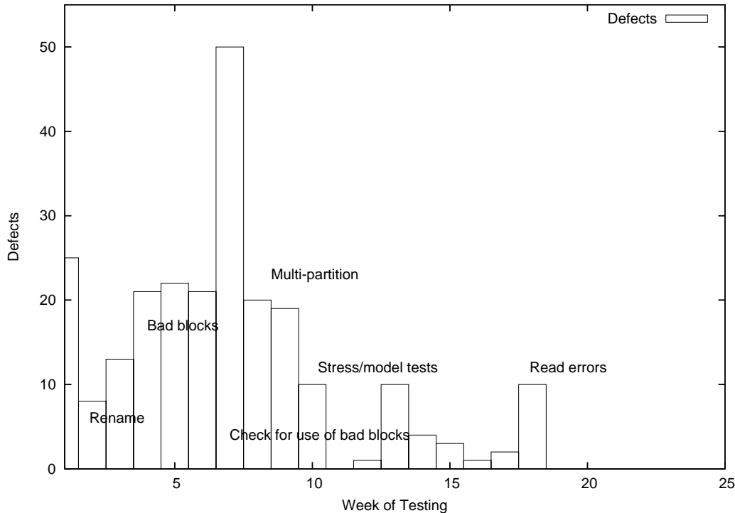
Figure 2. Results for the first 25 weeks of testing
